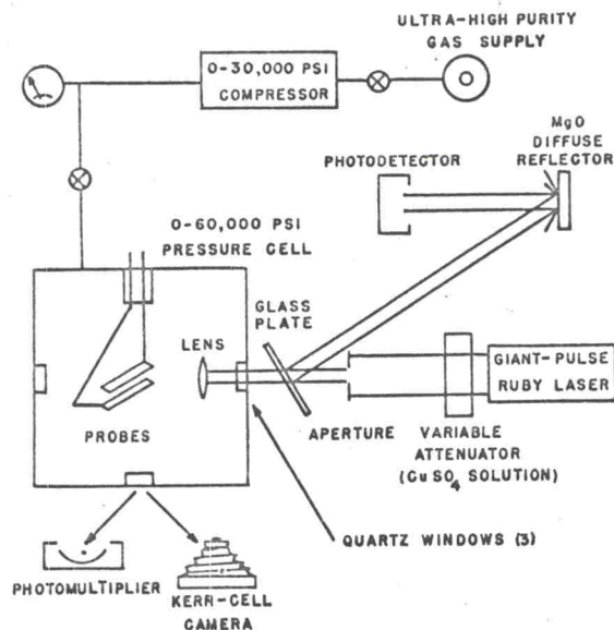
FIG. 1. Experimental apparatus for measurement of gas breakdown at super-high pressures using a focused laser beam.
